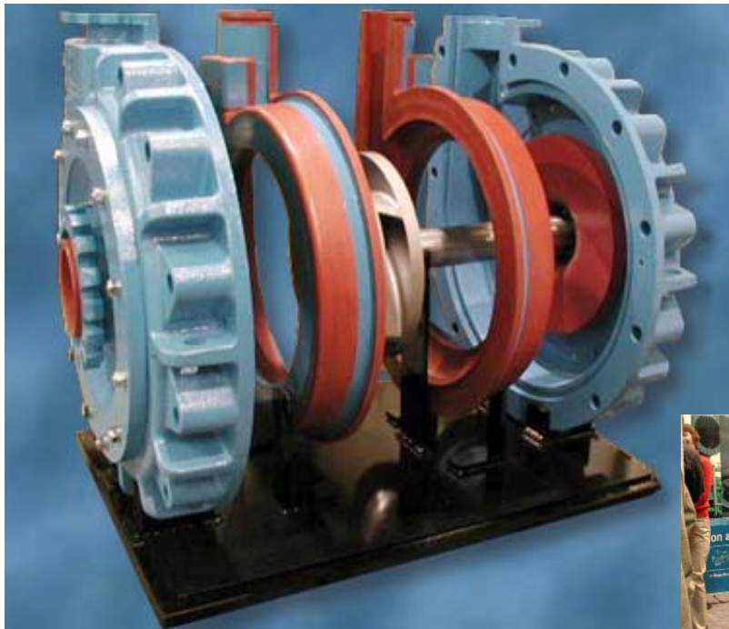
An exploded view is another fascinating way to show the inner workings of a product, and that was exactly what GIW had in mind.
